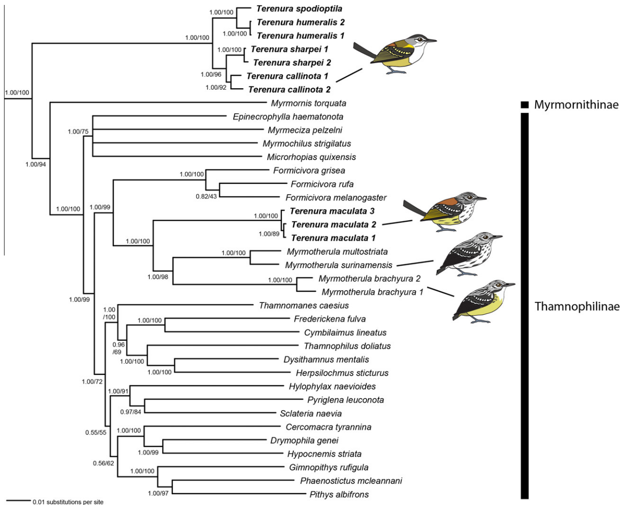
Fig. 1. 50% Majority-rule Bayesian consensus tree topology of a subset of the Thamnophilidae showing that Terenura callinota , T. humeralis , T. spodioptila , and T. sharpei are not closely related to T. maculata . Numbers at each node indicate posterior probability values (left) and bootstrap support values based on 1000 maximum-likelihood replicates (right). Outgroups not shown.
