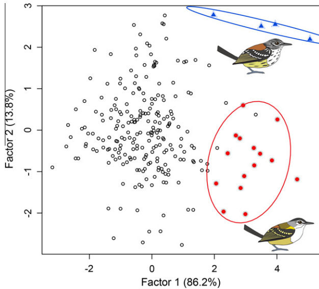
Fig. 2. Discriminant factors of ecomorphological variation of antwrens in the genera Epinecrophylla , Isteria , Myrmotherula , Microrhophias , Herpsilochmus , Formicivora , Stymphalornis , Terenura , and Euchrepomis . Positive values of Factor 1 represent shorter secondary 1 feathers. Positive values of Factor 2 represent shorter wings. Triangles represent specimens of Terenura . Solid circles represent specimens of Euchrepomis . Ellipses represent 95% confidence intervals.
