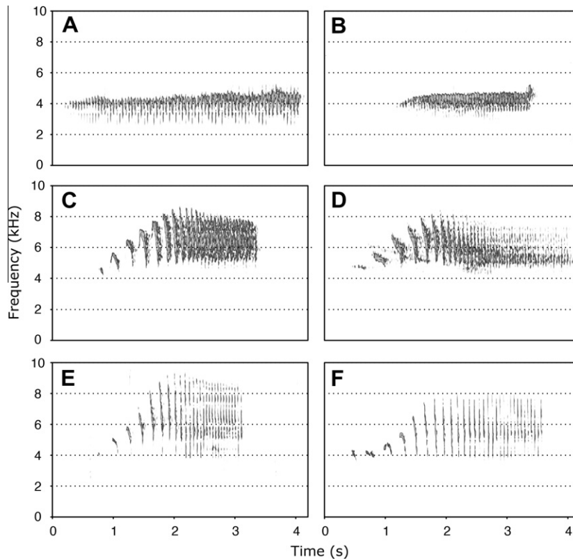
Fig. 3. Examples of loudsongs of Terenura (A – maculata ; B – sicki ) and Euchrepomis (C – callinota ; D – sharpei ; E – humeralis ; F – spodiopitla ). Both genera are characterized by remarkably high similarity of loudsongs among all of their respective species. Recordings obtained from Isler and Whitney (2002).
