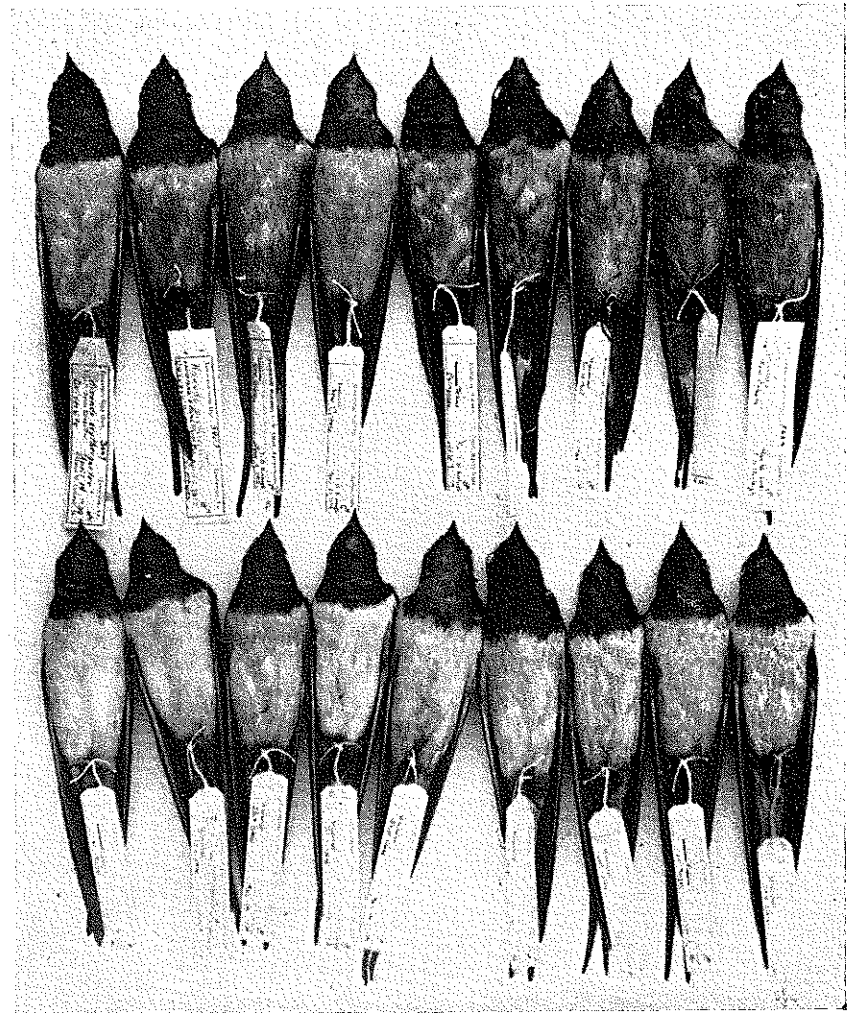
Photograph indicating the differences between males of Hirundo rustica erythrogaster (upper row) and Hirundo rustica insularis (bottom row). Made in daylight with Finopan (no filters) by J. Harvey Roberts.
